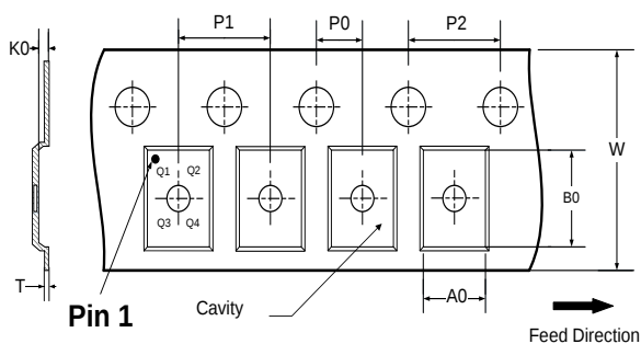
TAPE DIMENSIONS
